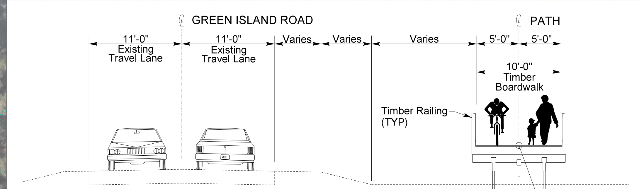
TYPICAL SECTION #3 GREEN ISLAND ROAD
