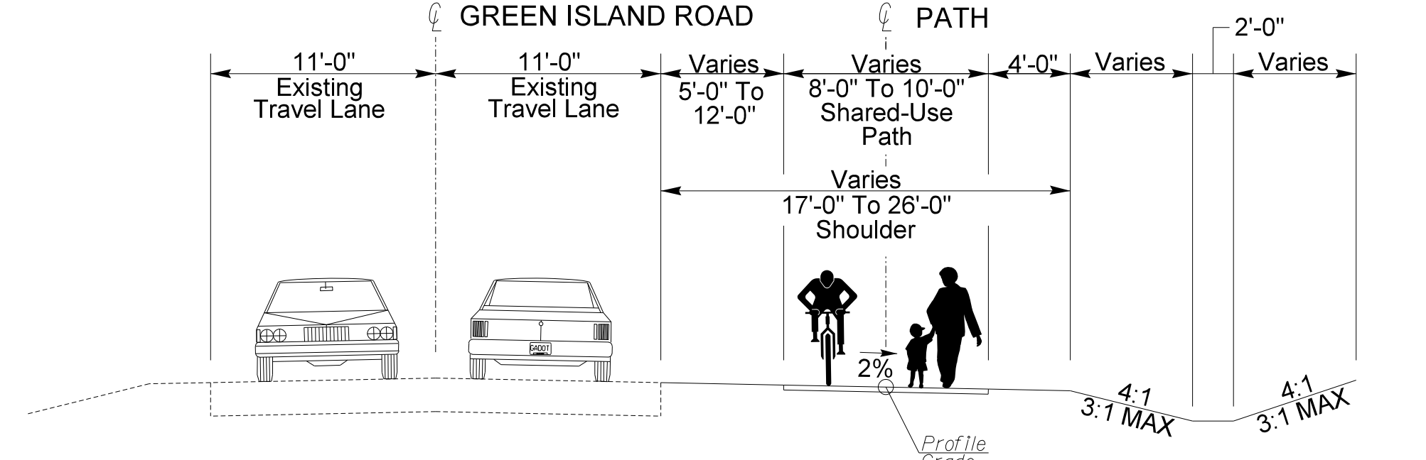
TYPICAL SECTION #4 GREEN ISLAND ROAD
