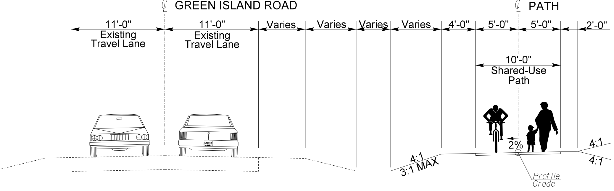
TYPICAL SECTION #2 GREEN ISLAND ROAD
